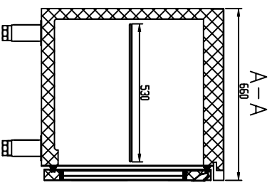
SECTION VIEW ?????
